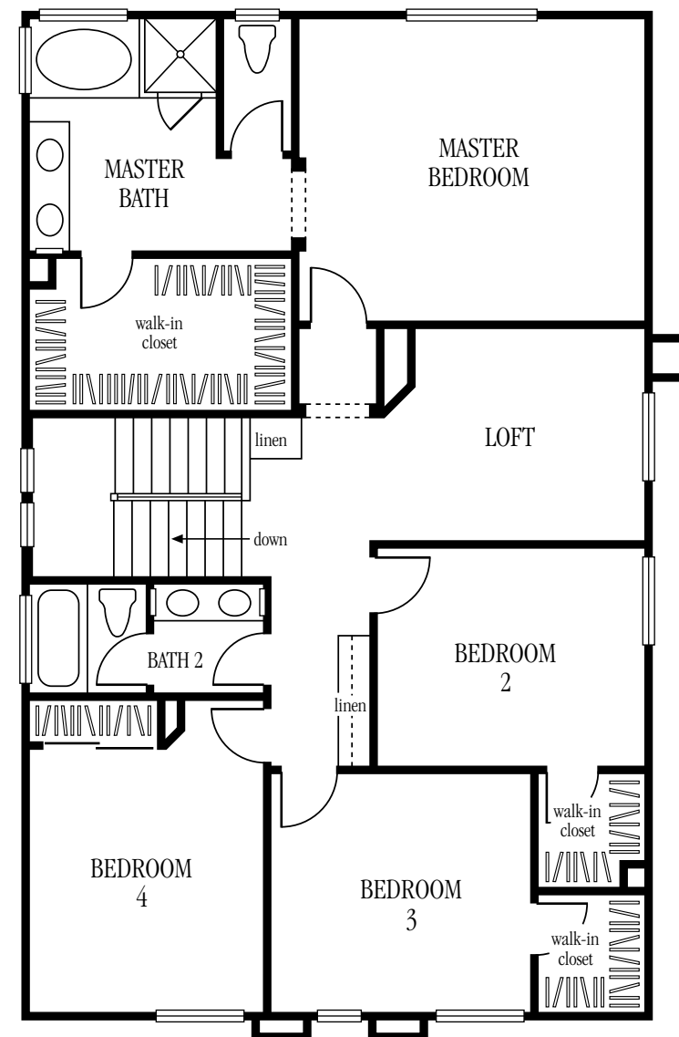
SECOND FLOOR
